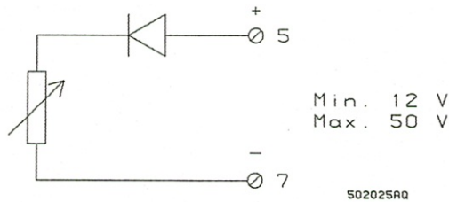
Fig. 4.1.a. Current output, schematic:
