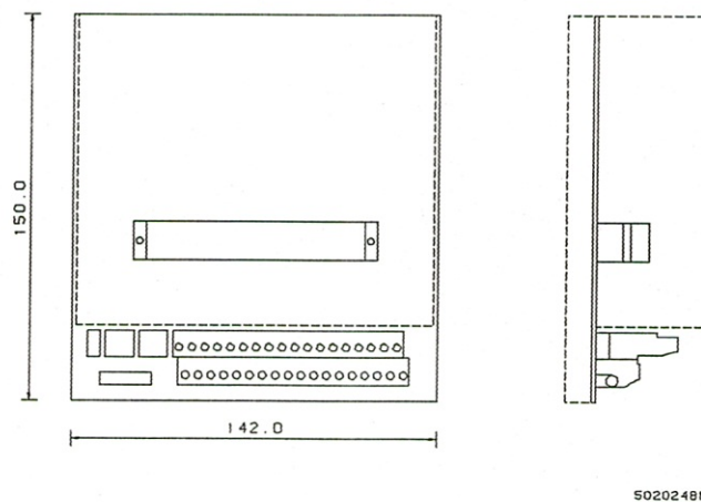
Fig 13.b: Base circuit board PD 1080
